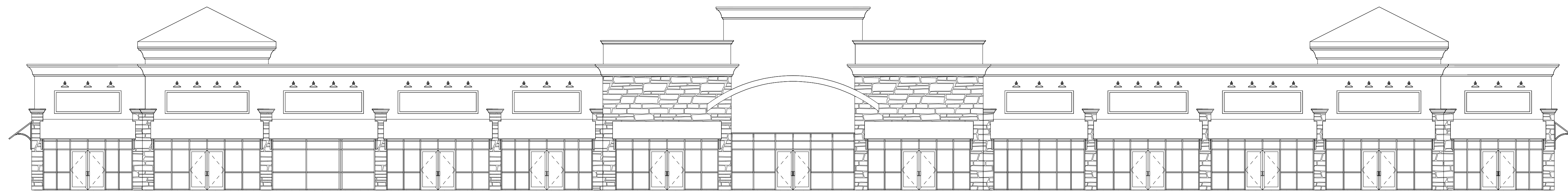
MAIN ELEVATION SCALE 1" = 10'-0"
